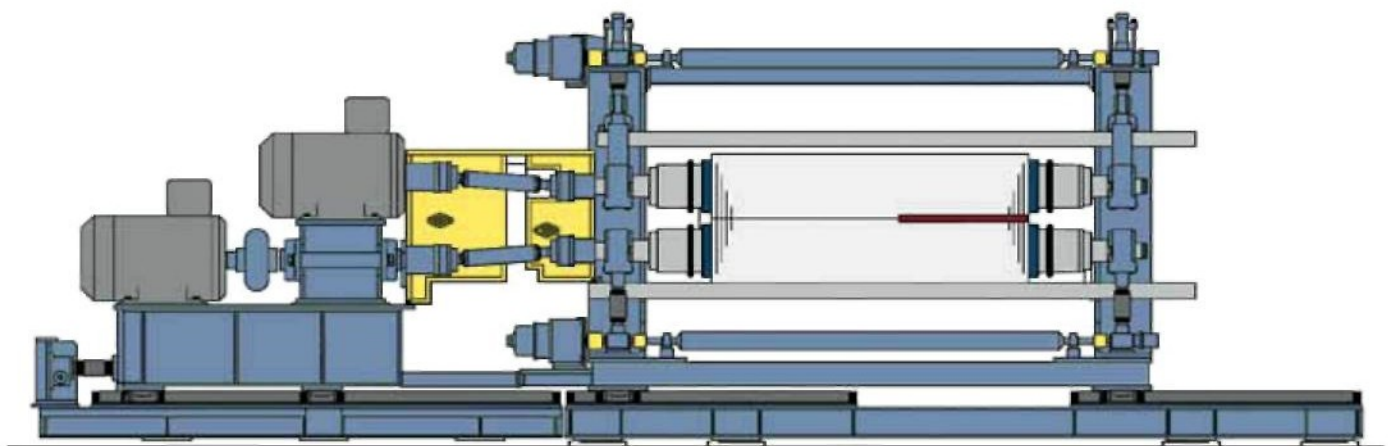
Brushing machine in brush / brush construction including oscillation
